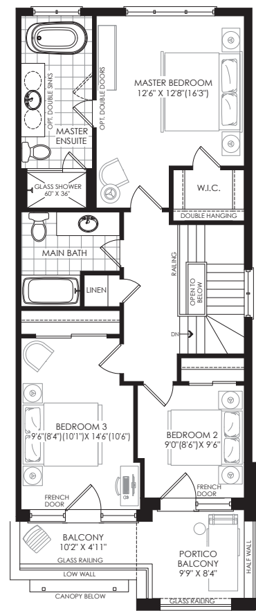
SECOND FLOOR PLAN ELEV. 'I'
