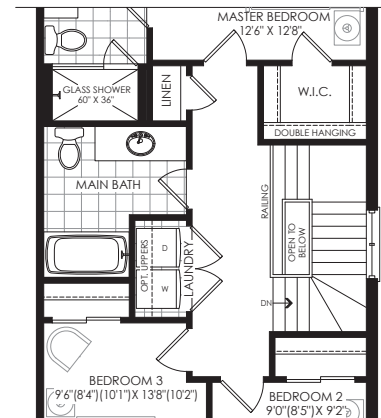
PARTIAL SECOND FLOOR FLEX PLAN WITH LAUNDRY
