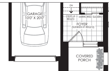
PARTIAL GROUND FLOOR ELEV. 'J'
