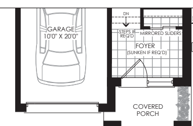
PARTIAL GROUND FLOOR ELEV. 'K'
