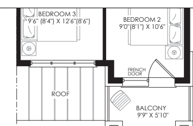
PARTIAL SECOND FLOOR PLAN ELEV. 'K'
